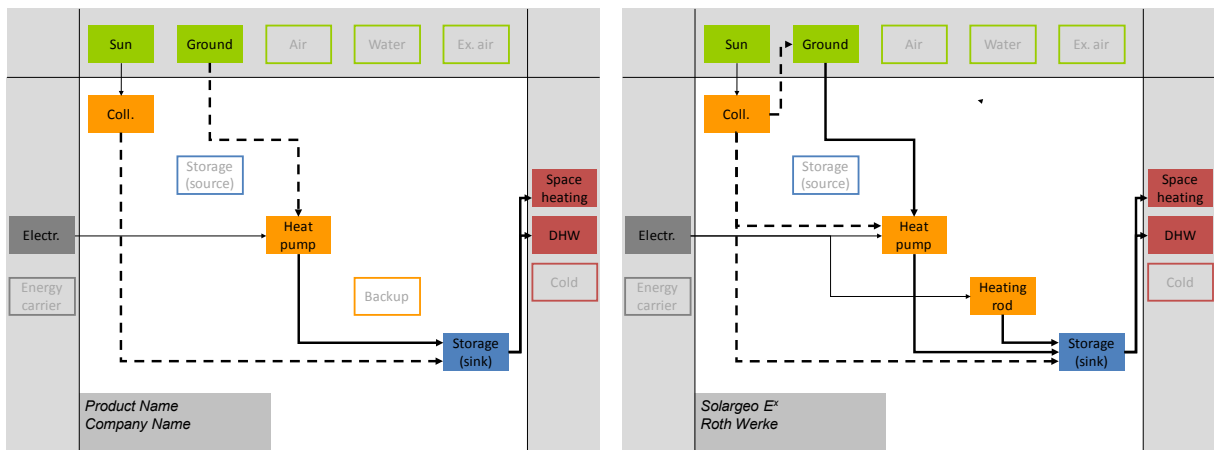
Fig. 2. Typical system with combistore (left) and “Solargeo E xx “ by Roth Werke (right)
