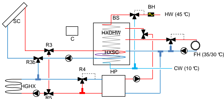
Fig. 2: Hydraulic scheme with solar thermal collectors (SC), ground heat exchanger (HGHX), heat pump (HP), buffer store (BS) with solar (HXSC)- and domestic hot water heat exchanger (HXDHW), direct electric backup-heater (BH), three-way-valves (R) as well as cold water (CW), hot water (HW), floor heating (FH) and controller (C)
