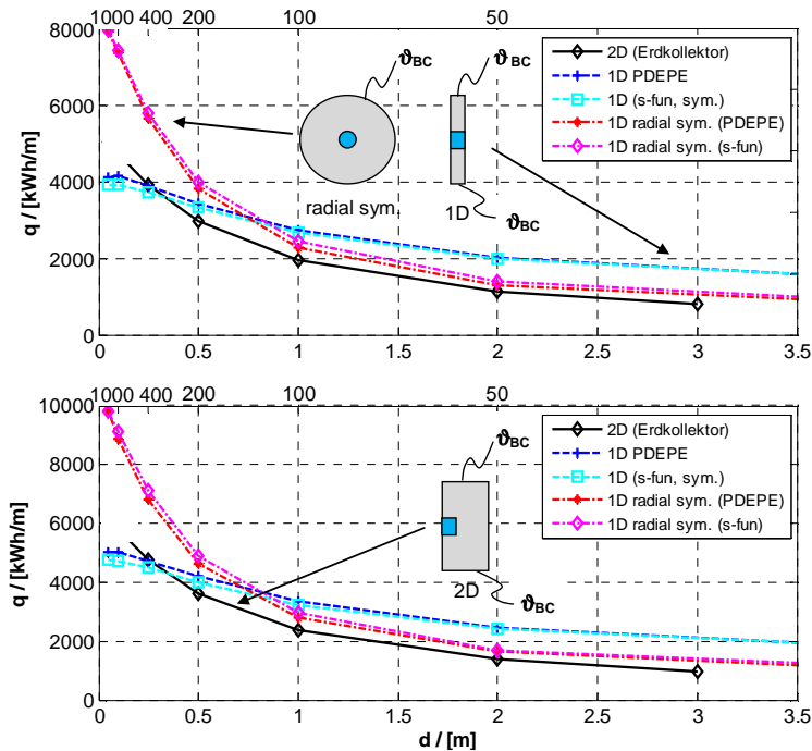
Fig. 6: Specific extraction heat (q) as a function of the pipe spacing (d) or the pipe length (L), respectively for a constant ground heat exchanger area of 100 m 2 ; Boundary and initial condition top: \vartheta_0 = \vartheta_{BC} = 10 °C and bottom: \vartheta_0 = \vartheta_{BC} = 8 °C; PE pipe DN 20, charging with V = 580 l/h, 40 % water glycol mixture
