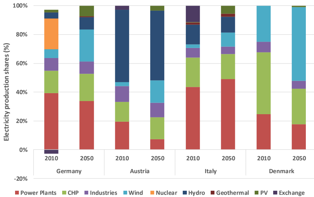
Figure 21: The proportion of electricity production from various technologies in the four countries in the 2010 and 2050 models The electricity production per capita is 6-10 MWh/capita/year in 2010 and is expected to increase towards 2050 in all countries. Austria has the highest production per capita which indicates that the energy system to a larger degree is based on electricity than in the other countries.
