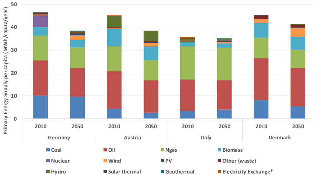
Figure 20: The primary energy supply per capita for the different countries in the 2010 and 2050 models.
