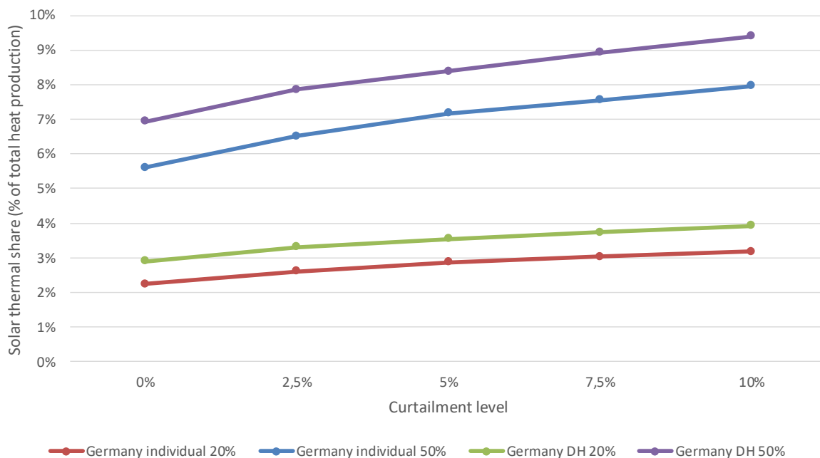
Figure 68: Solar thermal share of heat production at different overproduction levels. The figure shows that the difference in terms of solar thermal share is around one percentage point when increasing the overproduction level from 5% to 10% with a high solar penetration rate and around half a percentage point when the solar penetration rate is lower.
