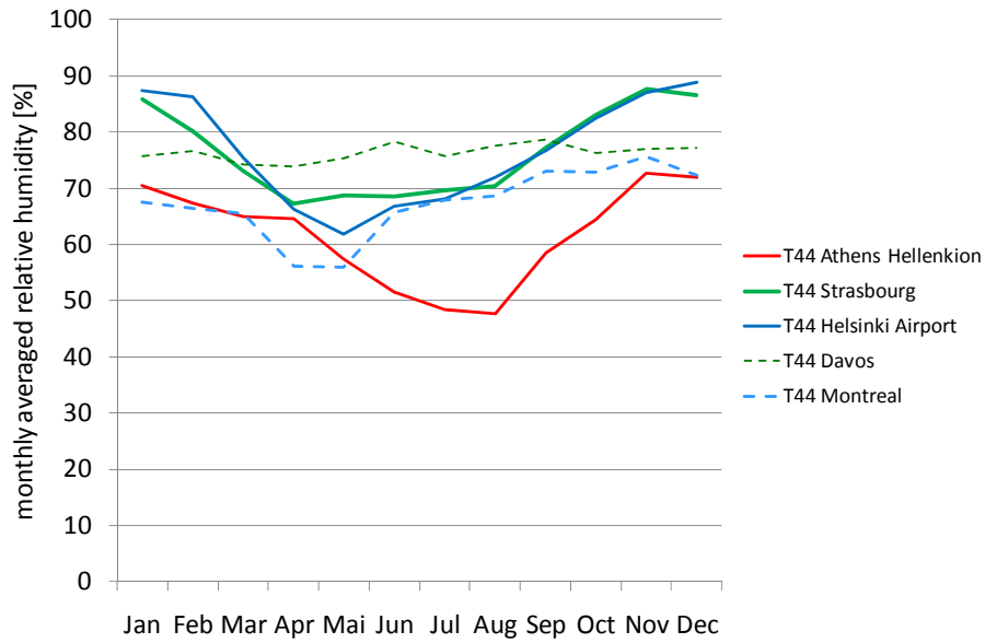
Figure 3: Comparison of monthly averaged relative humidity for the Task 44 climate data of Strasbourg, Athens, Helsinki and Davos. No relative humidity data is available from (EC 2010/30/EU 2010).
