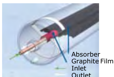
Fig. 7: Function and design of the Lenz tube [4]
